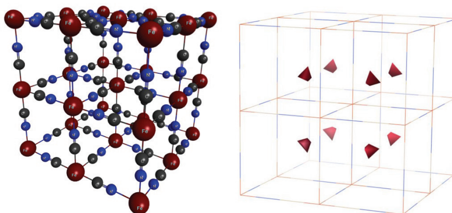
Figure 1: Structure of PB nanoparticle (left) and isosurface plot of Cs + distribution (right).
